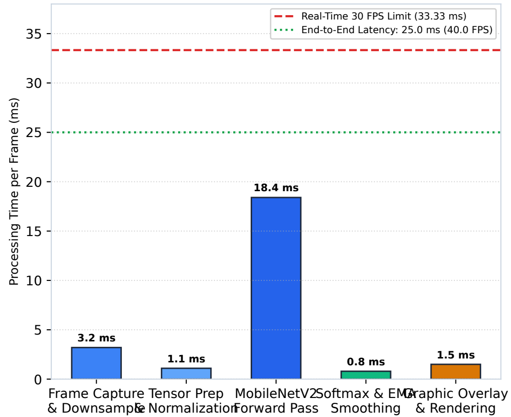
Figure 7(b): Real-Time Inference Latency Breakdown (Total: 25.0 ms/frame = 40.0 FPS, 25.0% Safety Headroom)
